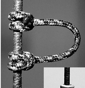
Nocking loop with ends terminating on opposite sides of string.
